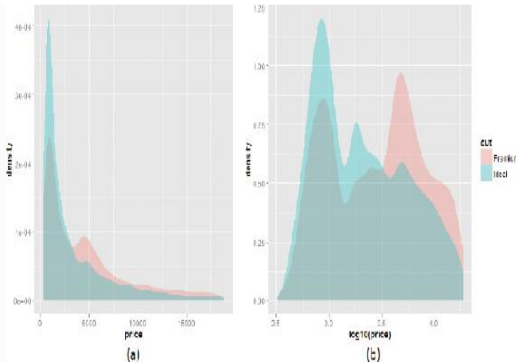
FIGURE 3-12 Density plots of (a) diamond prices and (b) the logarithm of diamond prices
