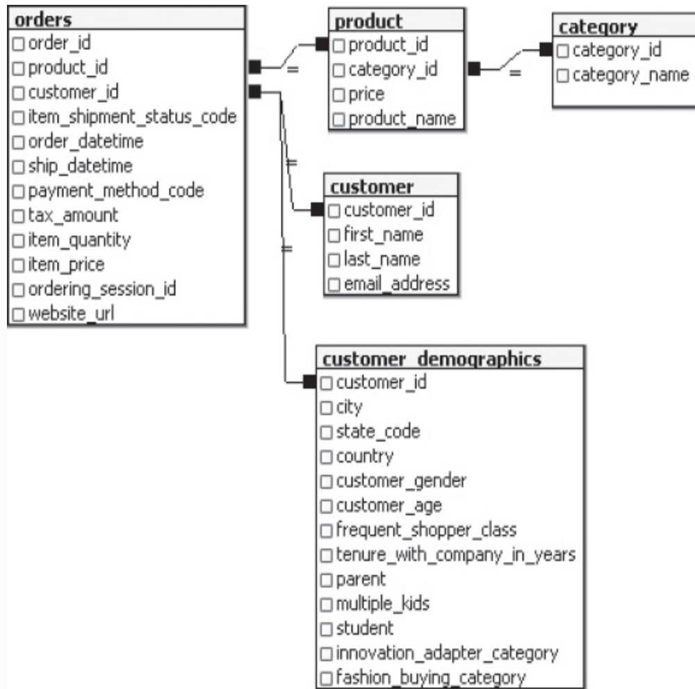
FIGURE 11-1 Relationship diagram
