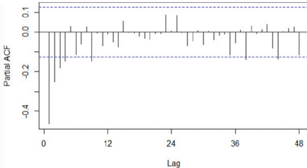
FIGURE 8-16 PACF of residuals from seasonal AR(1) model
