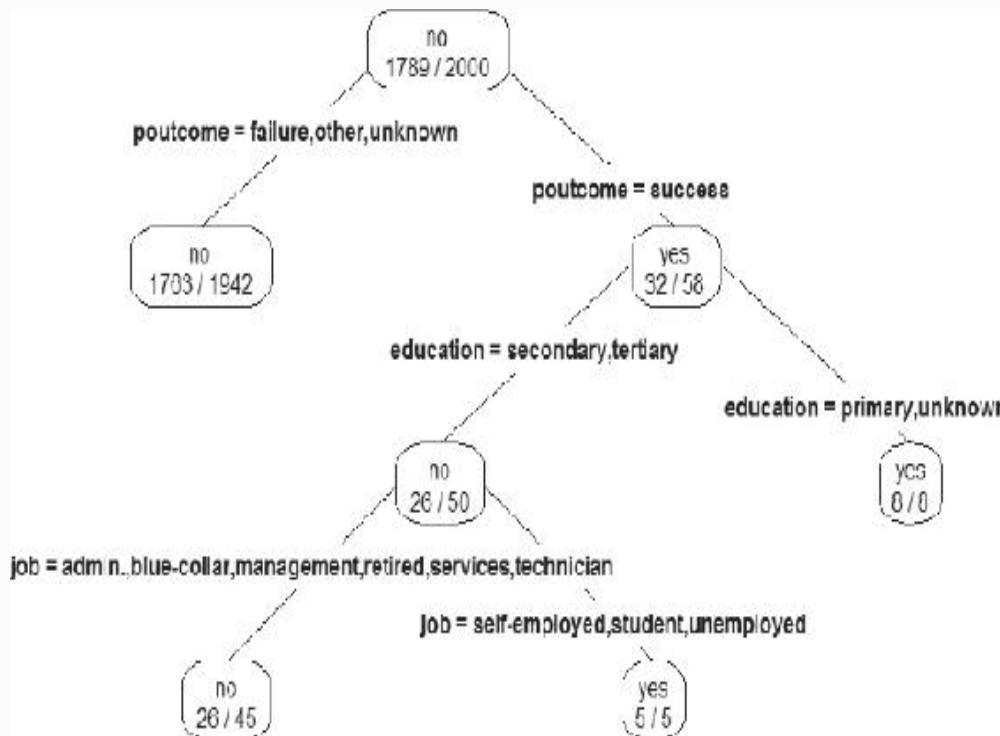
FIGURE 7-4 Using a decision tree to predict if a client will subscribe to a term deposit
