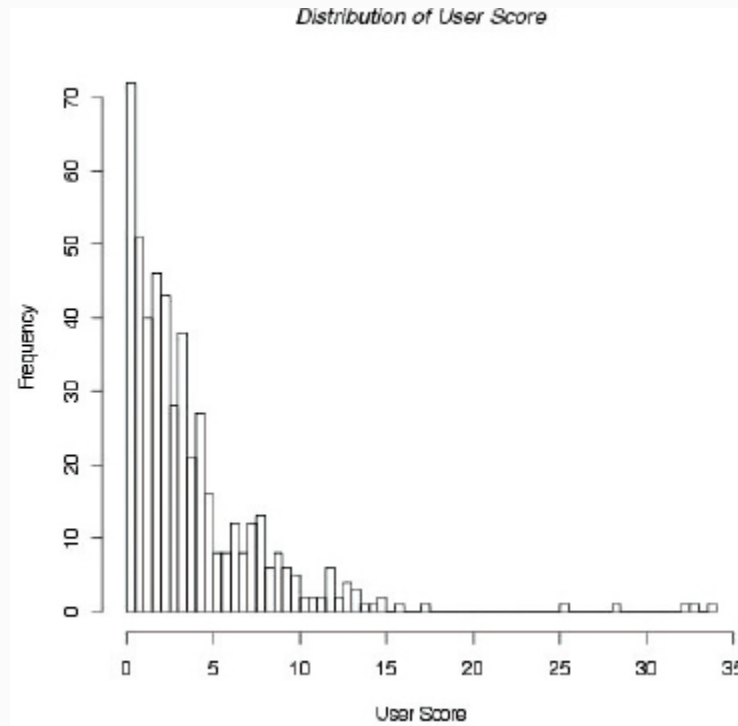
FIGURE 12-19 Frequency distribution of user scores
