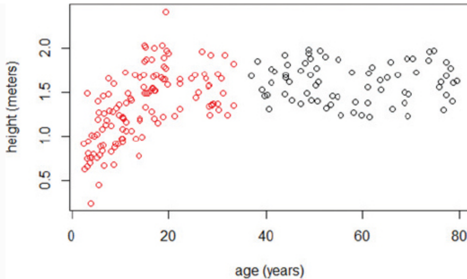
FIGURE 4-12 Clusters with height expressed in meters
