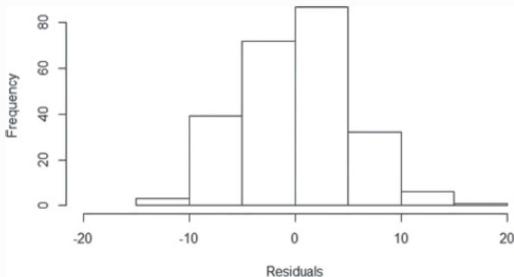
FIGURE 8-20 Histogram of the residuals from the fitted (0,1,1) \times (1,0,0)_{12} model
