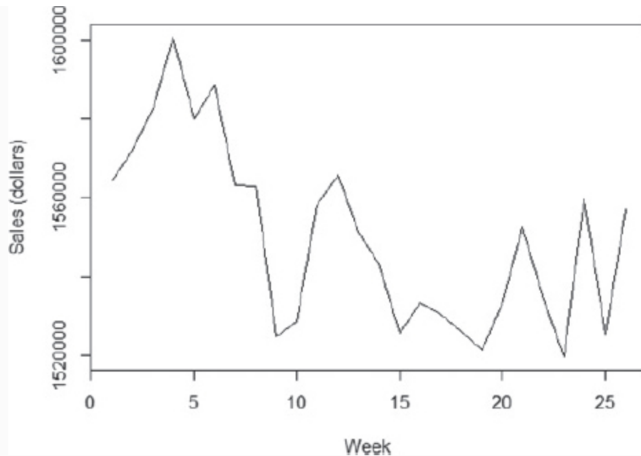
FIGURE 11-2 Weekly sales for an online retailer
