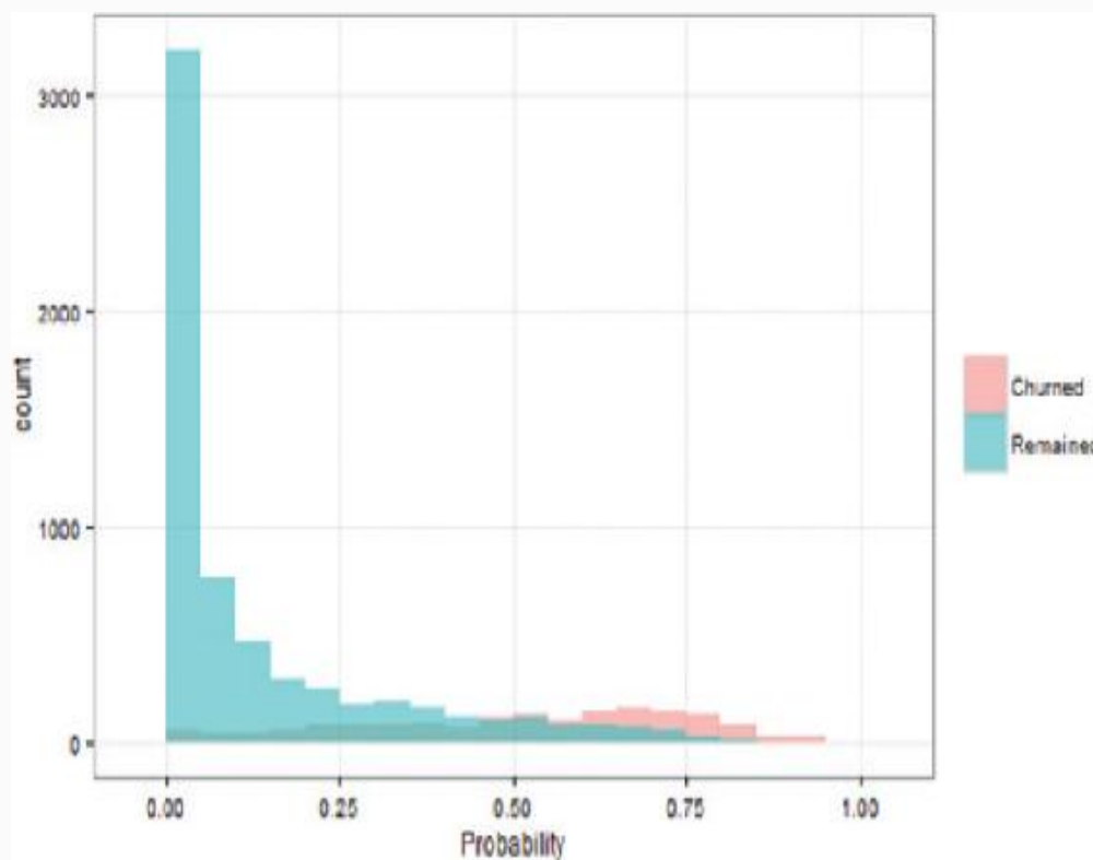
FIGURE 6-17 Customer counts versus estimated churn probability
