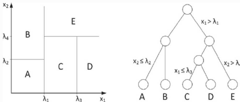
FIGURE 7-8 Decision surfaces can only be axis-aligned
