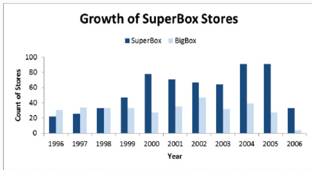
FIGURE 12-34 Simple bar chart, with two dimensions
