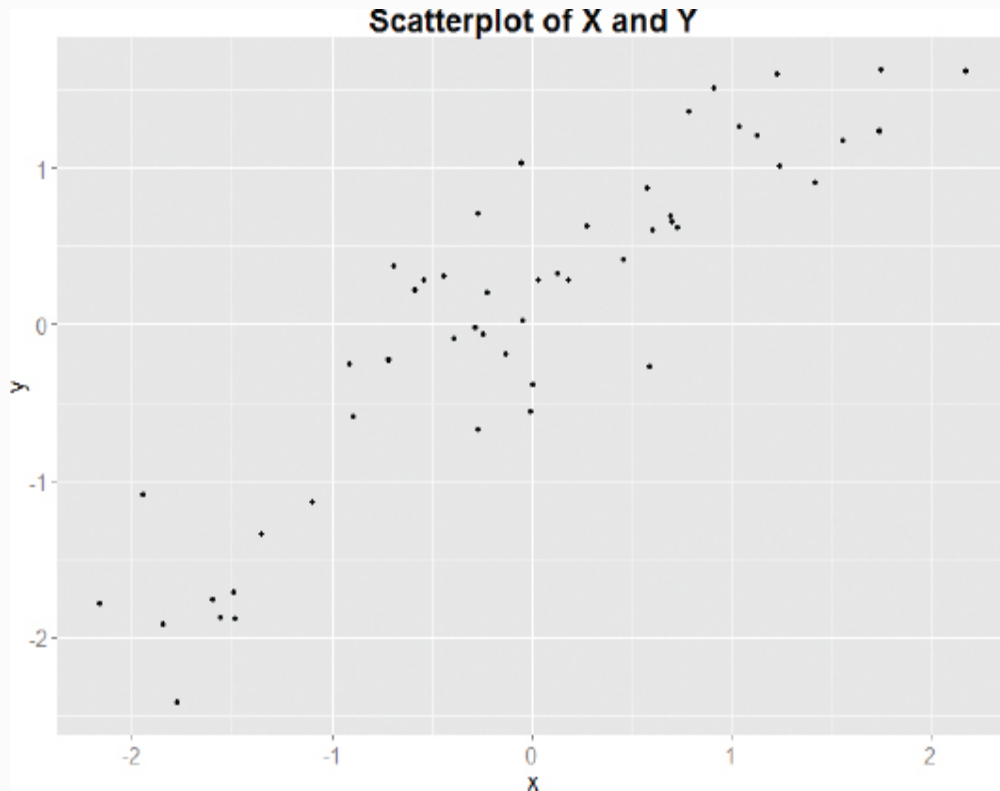
FIGURE 3-5 A scatterplot can easily show if x and y share a relation
