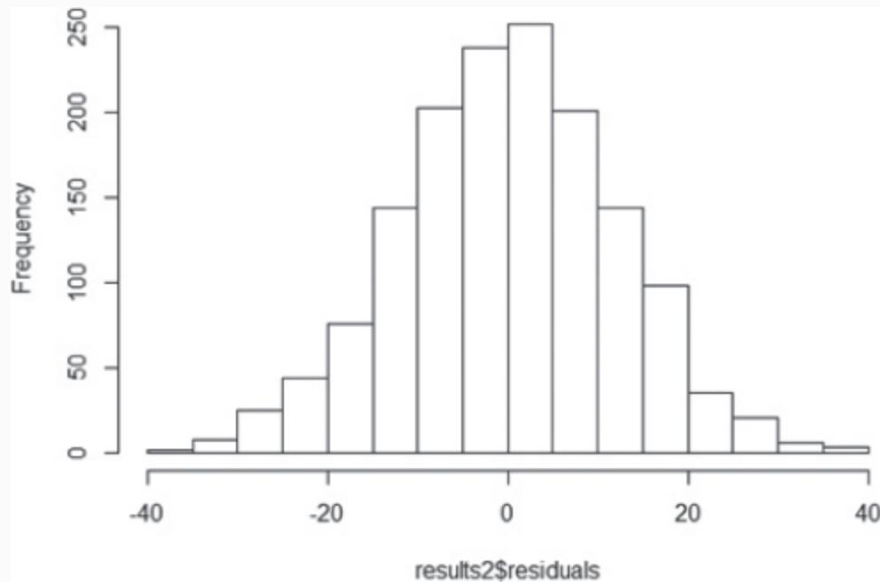
FIGURE 6-11 Histogram of normally distributed residuals
