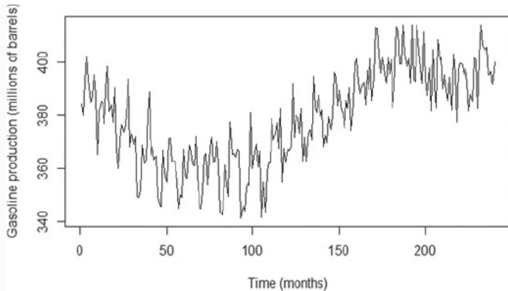
FIGURE 8-11 Monthly gasoline production
