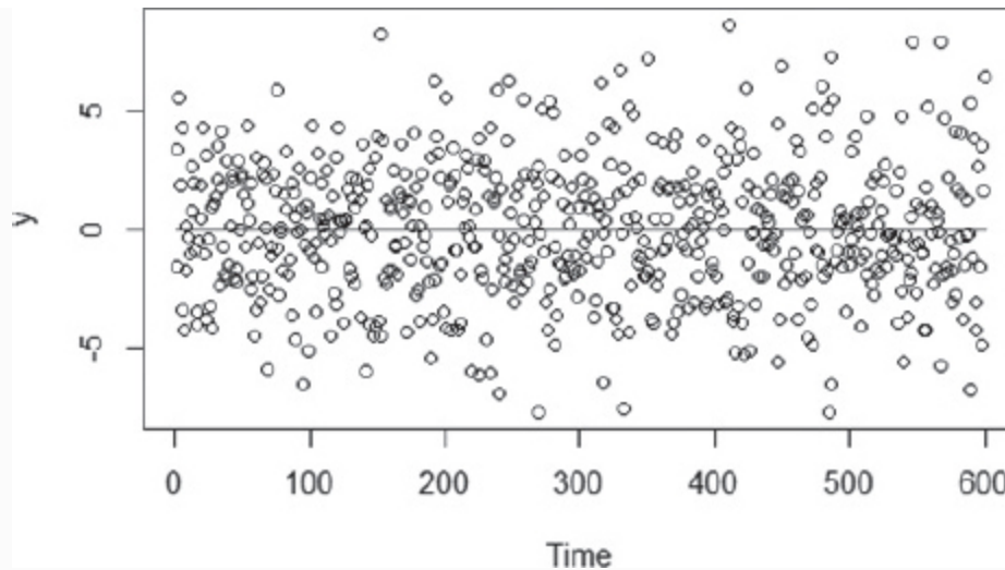
FIGURE 8-5 Scatterplot of a simulated MA(3) time series
