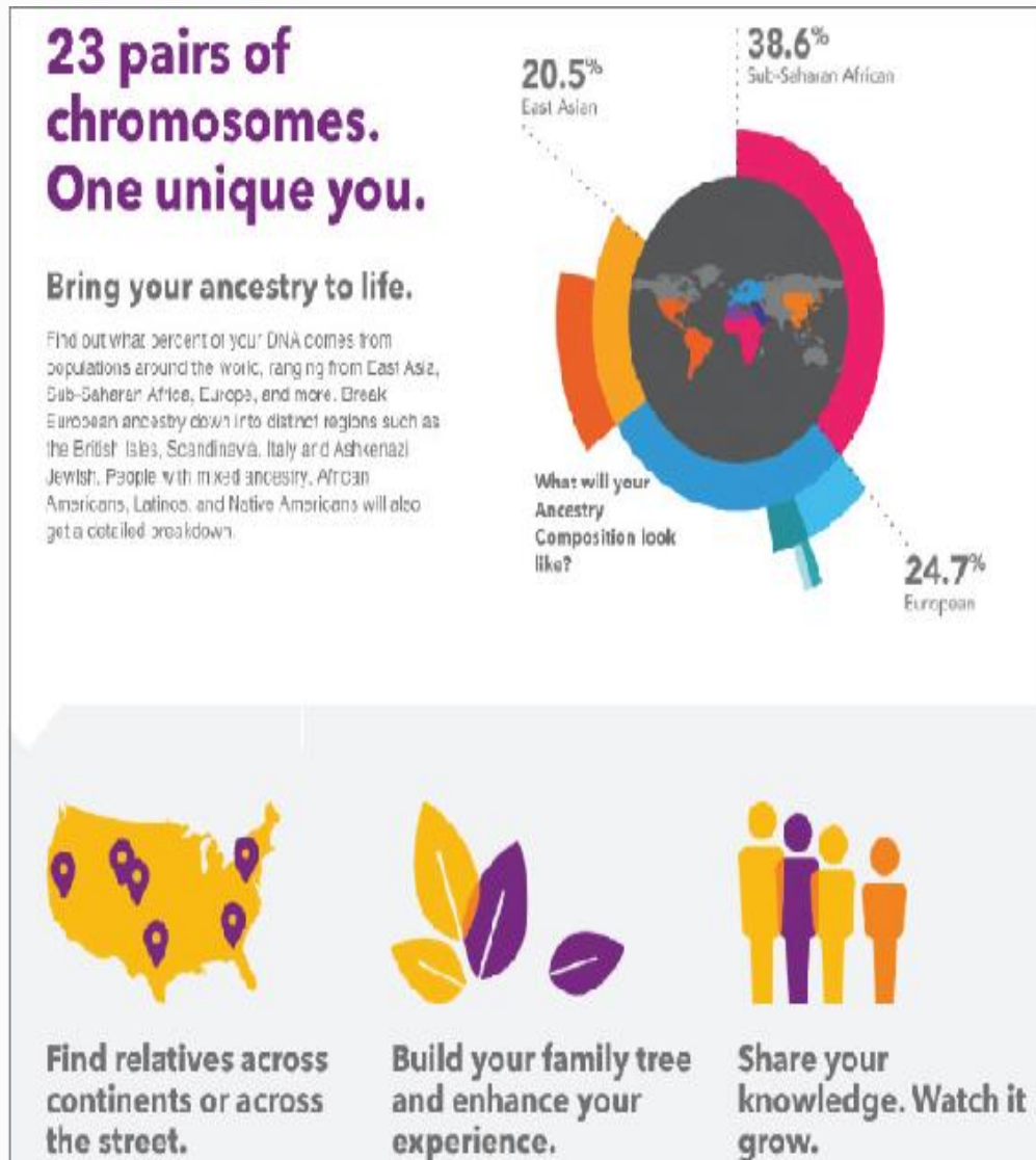
FIGURE 1-2 Examples of what can be learned through genotyping, from 23andme.com
