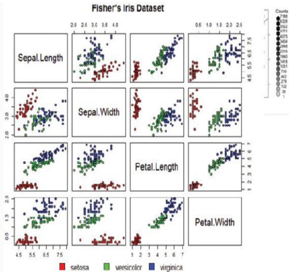
FIGURE 3-18 Scatterplot matrix of Fisher's [13] iris dataset
