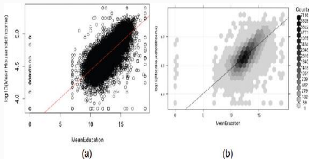
FIGURE 3-17 (a) Scatterplot and (b) Hexbinplot of household income against years of education
