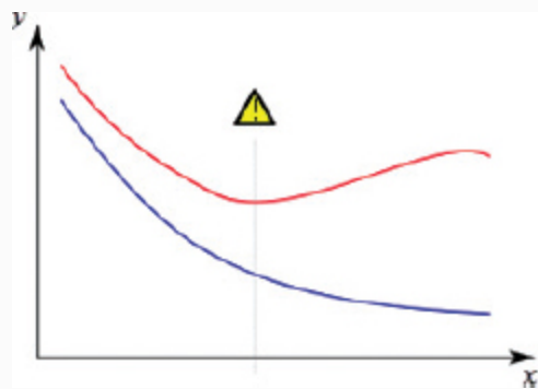
FIGURE 7-7 An overfit model describes the training data well but predicts poorly on unseen data
