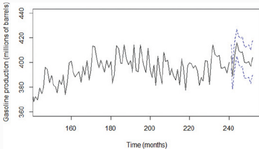
FIGURE 8-22 Actual and forecasted gasoline production
