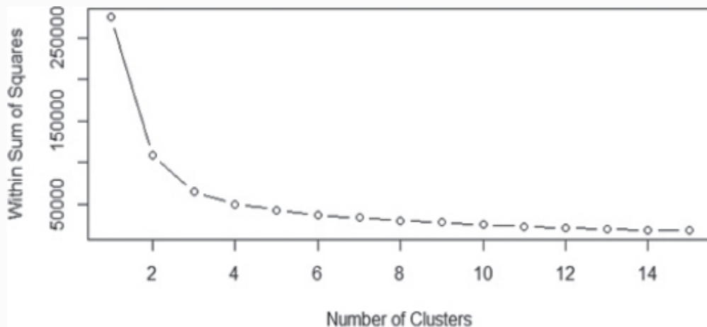
FIGURE 4-5 WSS of the student grade data
