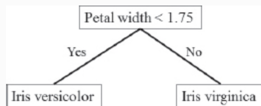
FIGURE 7-2 Example of a decision stump
