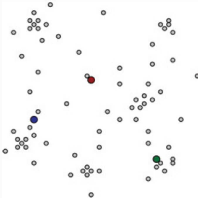
FIGURE 4-2 Initial starting points for the centroids
