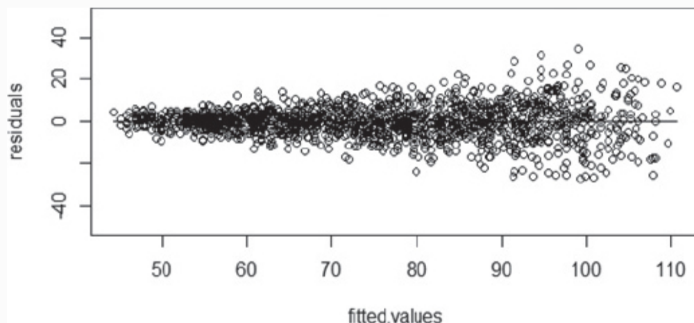
FIGURE 6-9 Residuals with a linear trend
