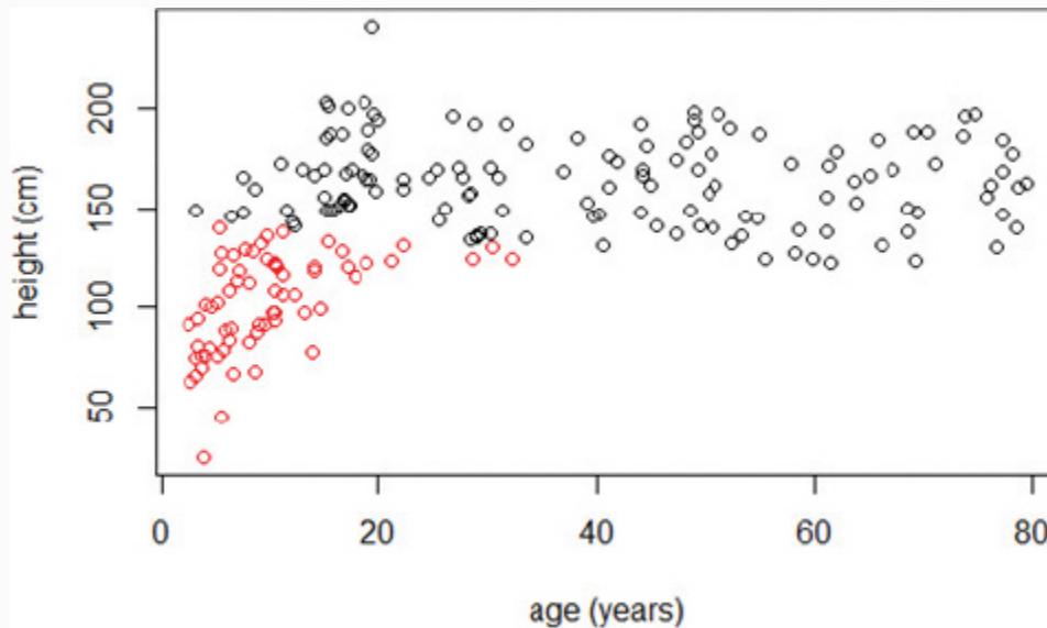
FIGURE 4-11 Clusters with height expressed in centimeters
