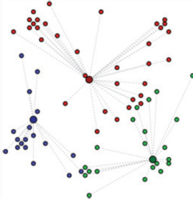
FIGURE 4-3 Points are assigned to the closest centroid
