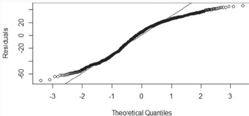
FIGURE 6-13 Q-Q plot of non-normally distributed residuals
