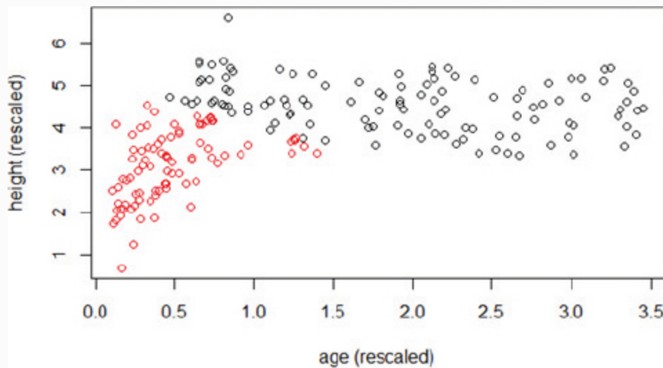
FIGURE 4-13 Clusters with rescaled attributes
