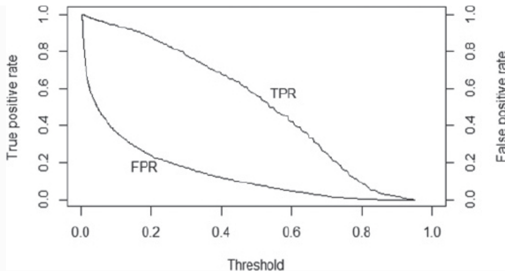
FIGURE 6-16 The effect of the threshold value in the churn example
