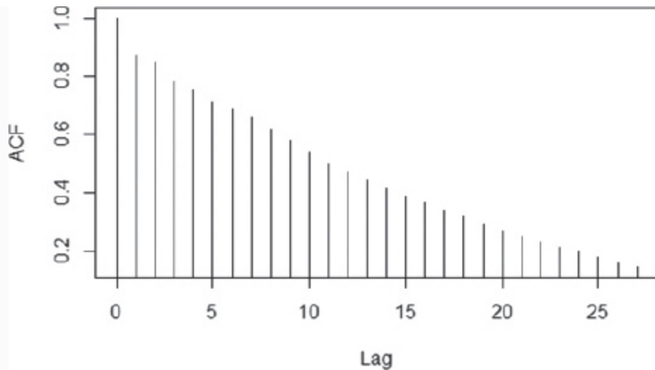
FIGURE 8-3 Autocorrelation function (ACF)
