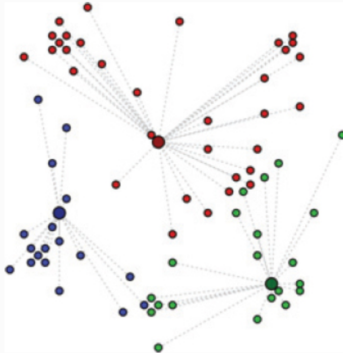
FIGURE 4-1 Possible k -means clusters for k=3
