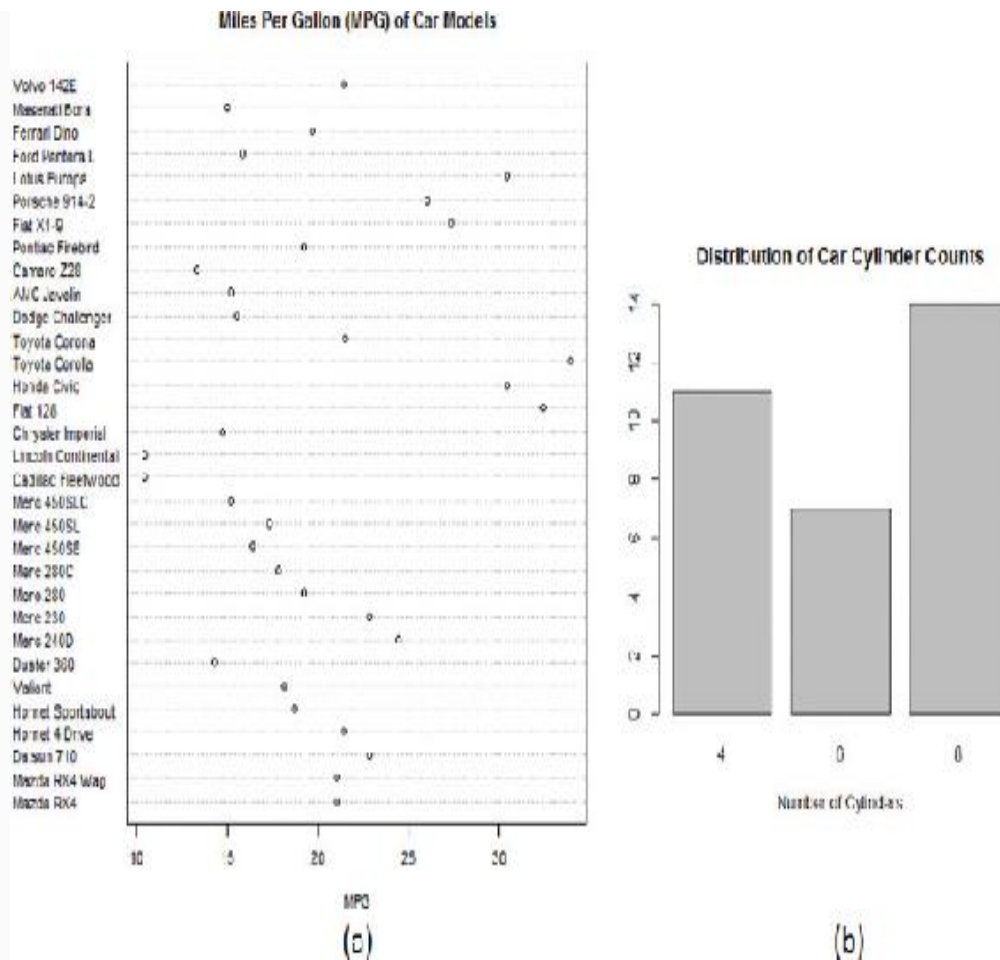
FIGURE 3-10 (a) Dotchart on the miles per gallon of cars and (b) Barplot on the distribution of car cylinder counts
