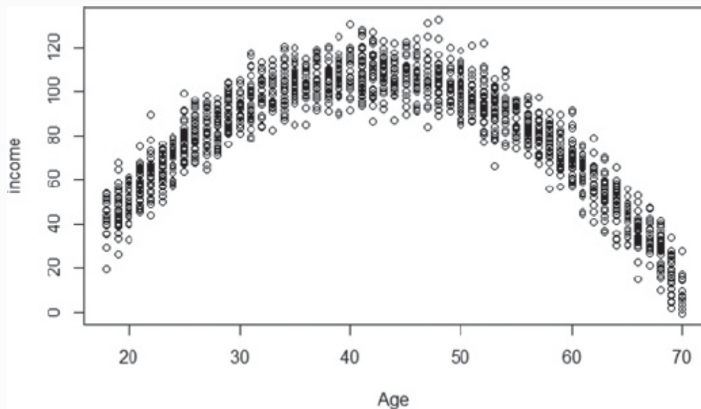
FIGURE 6-5 Income as a quadratic function of Age
