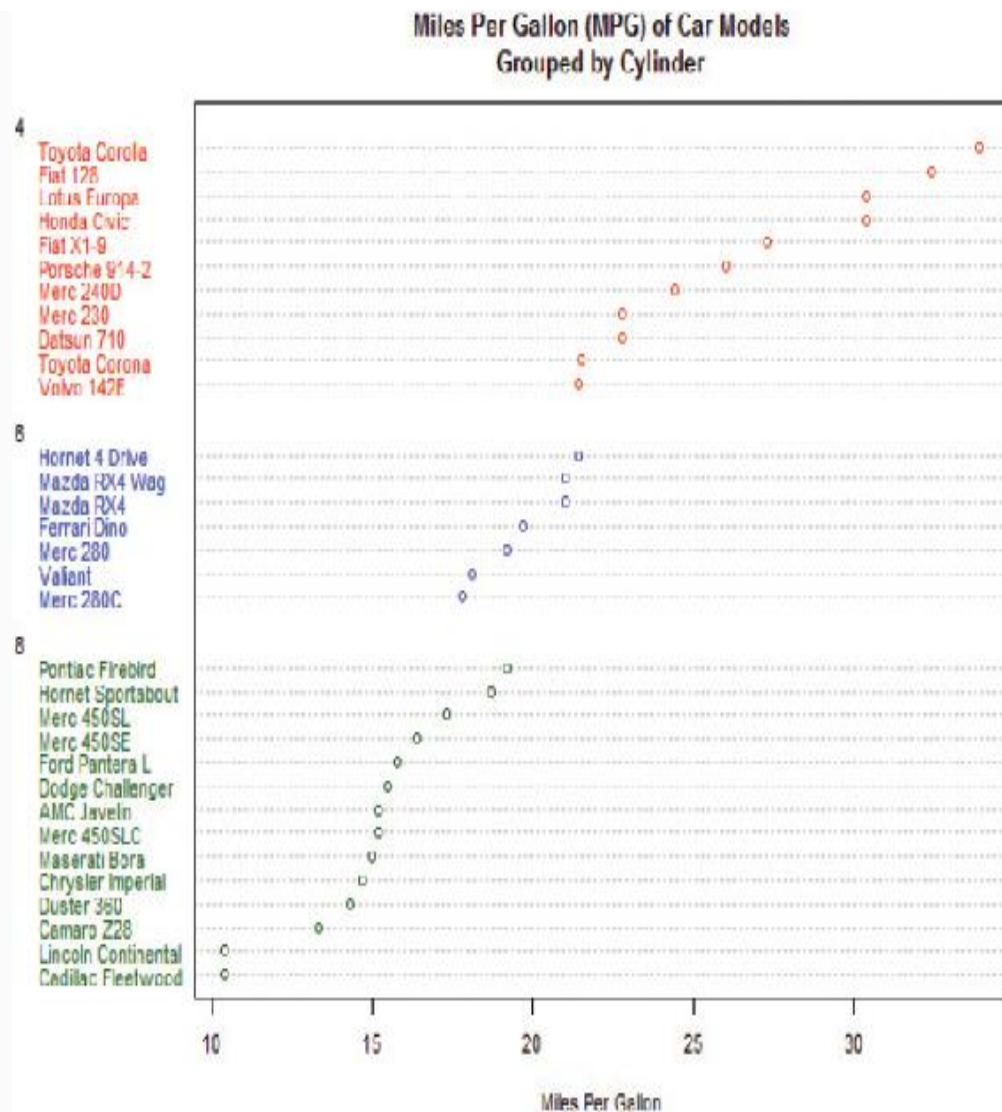
FIGURE 3-14 Dotplot to visualize multiple variables
