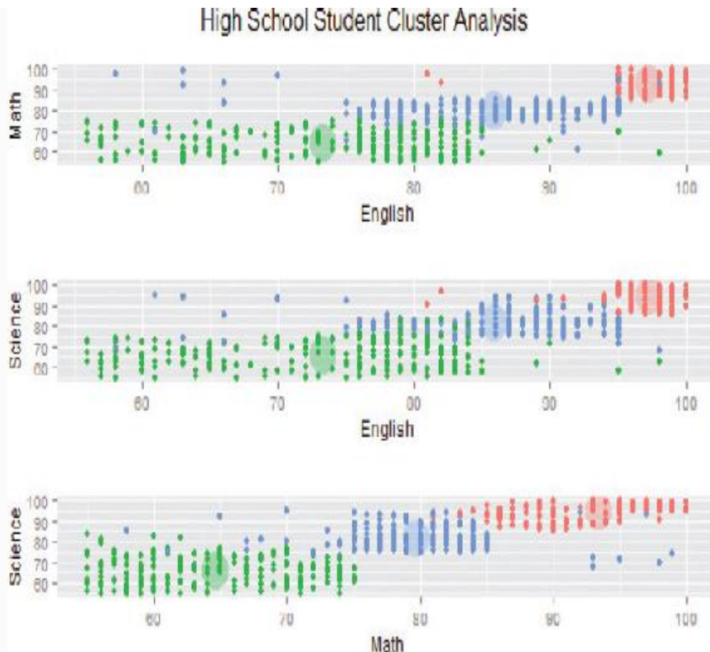
FIGURE 4-6 Plots of the identified student clusters
