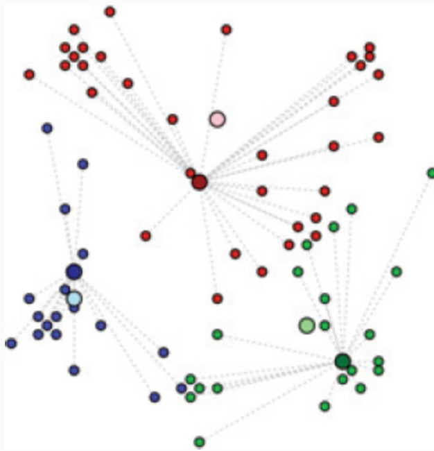
FIGURE 4-4 Compute the mean of each cluster
