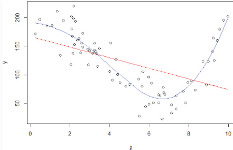
FIGURE 3-13 Examining two variables with regression
