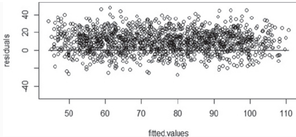
FIGURE 6-8 Residuals not centered on the zero line
