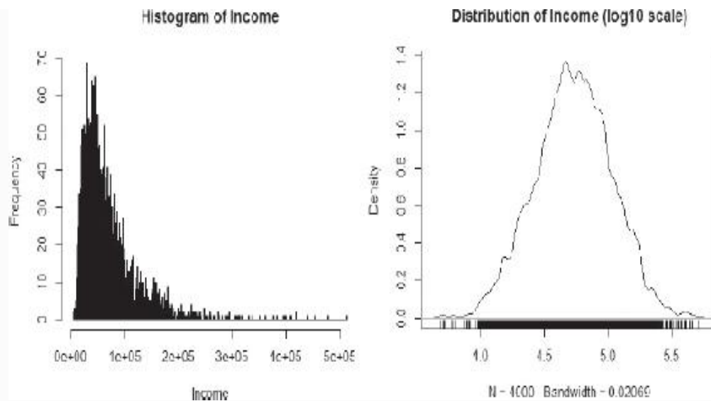
FIGURE 3-11 (a) Histogram and (b) Density plot of household income
