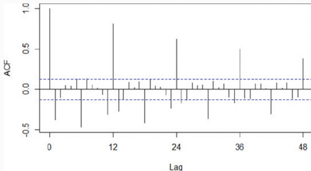
FIGURE 8-13 ACF of the differenced gasoline time series
