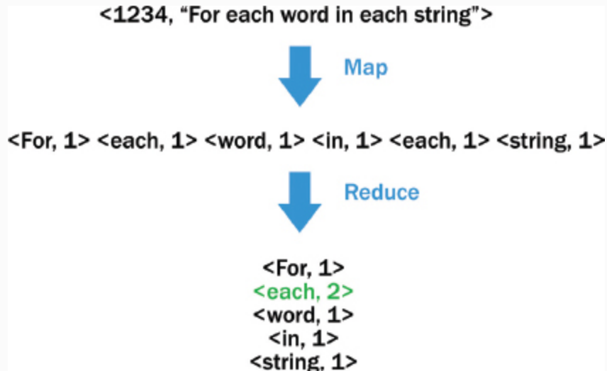
FIGURE 10-1 Example of how MapReduce works
