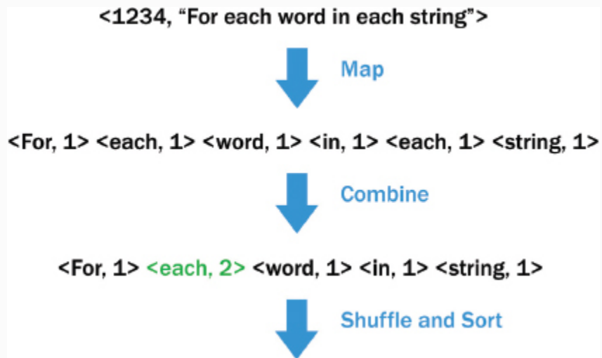
FIGURE 10-4 Using a combiner
