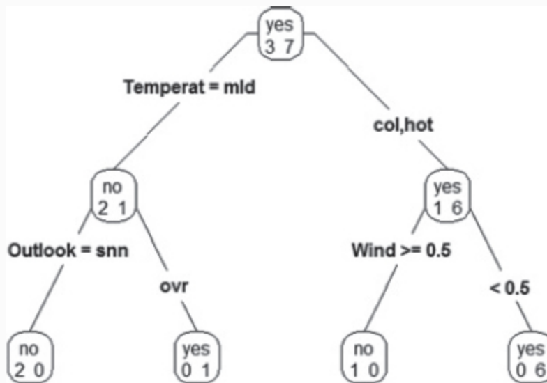
FIGURE 7-9 A decision tree built from DTdata.csv
