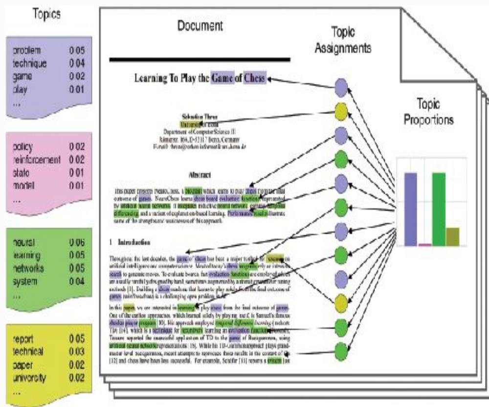
FIGURE 9-4 The intuitions behind LDA
