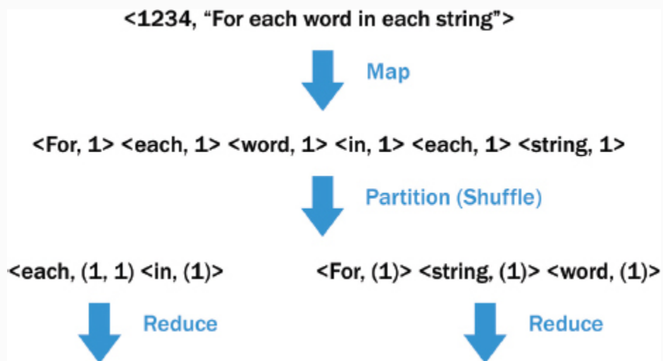
FIGURE 10-5 Using a custom partitioner
