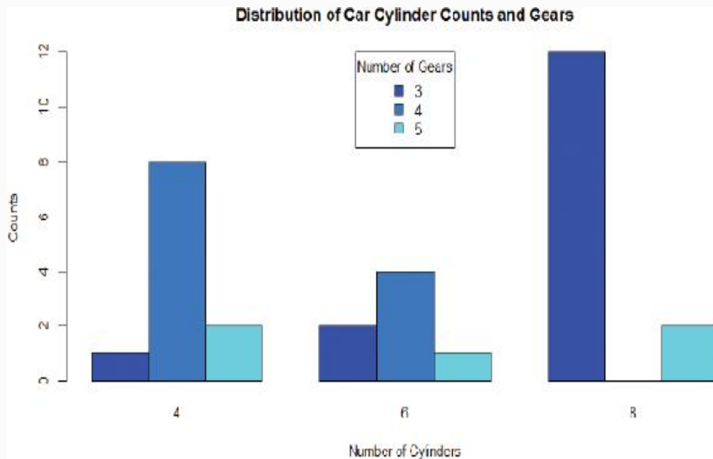
FIGURE 3-15 Barplot to visualize multiple variables
