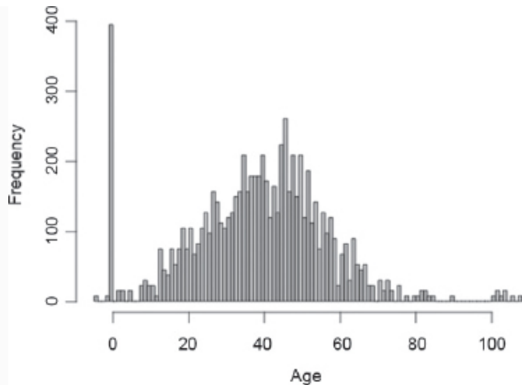
FIGURE 3-8 Age distribution of bank account holders
