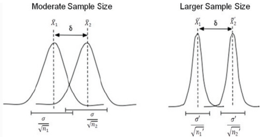
FIGURE 3-26 A larger sample size better identifies a fixed effect size
