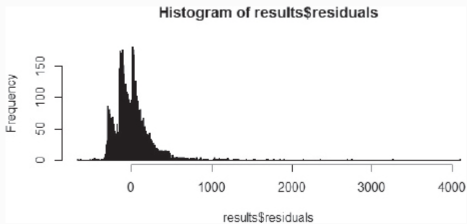
FIGURE 3-2 Evidence of large residuals
