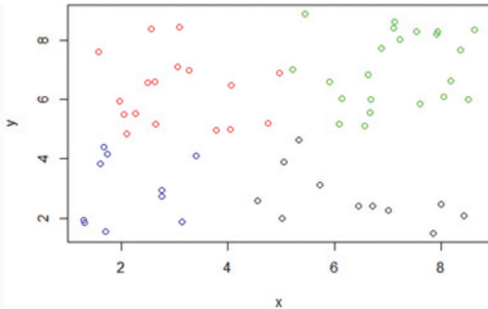
FIGURE 4-8 Example of less obvious clusters
