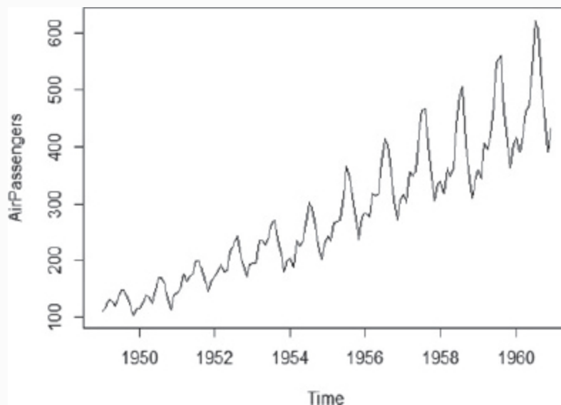
FIGURE 3-19 Airline passenger counts from 1949 to 1960
