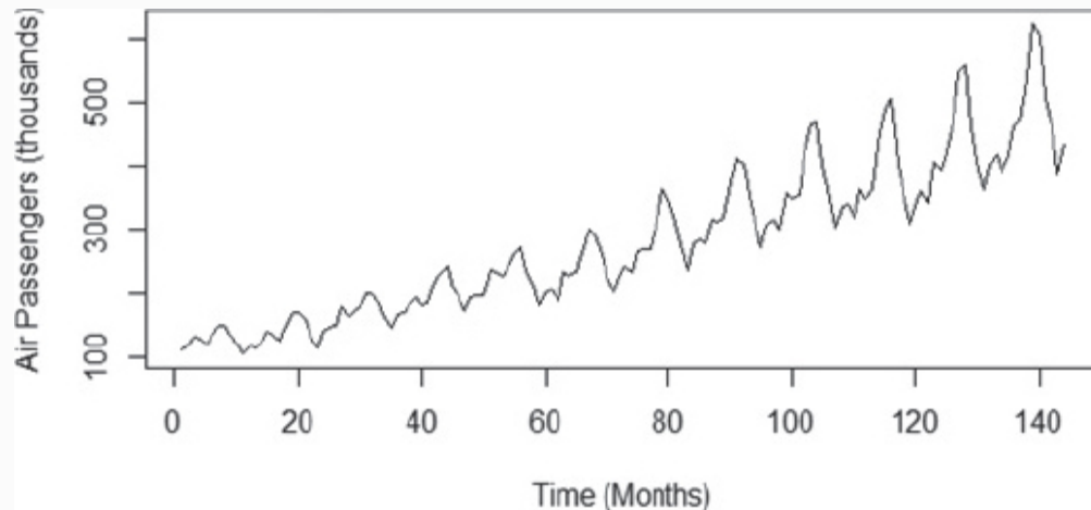
FIGURE 8-1 Monthly international airline passengers
