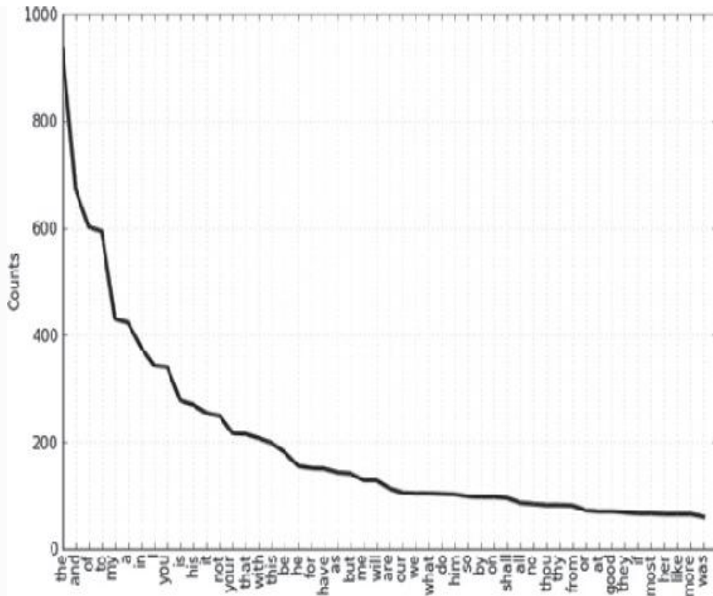
FIGURE 9-2 The 50 most frequent words in Shakespeare's Hamlet
