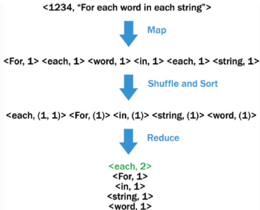
FIGURE 10-3 Shuffle and sort
