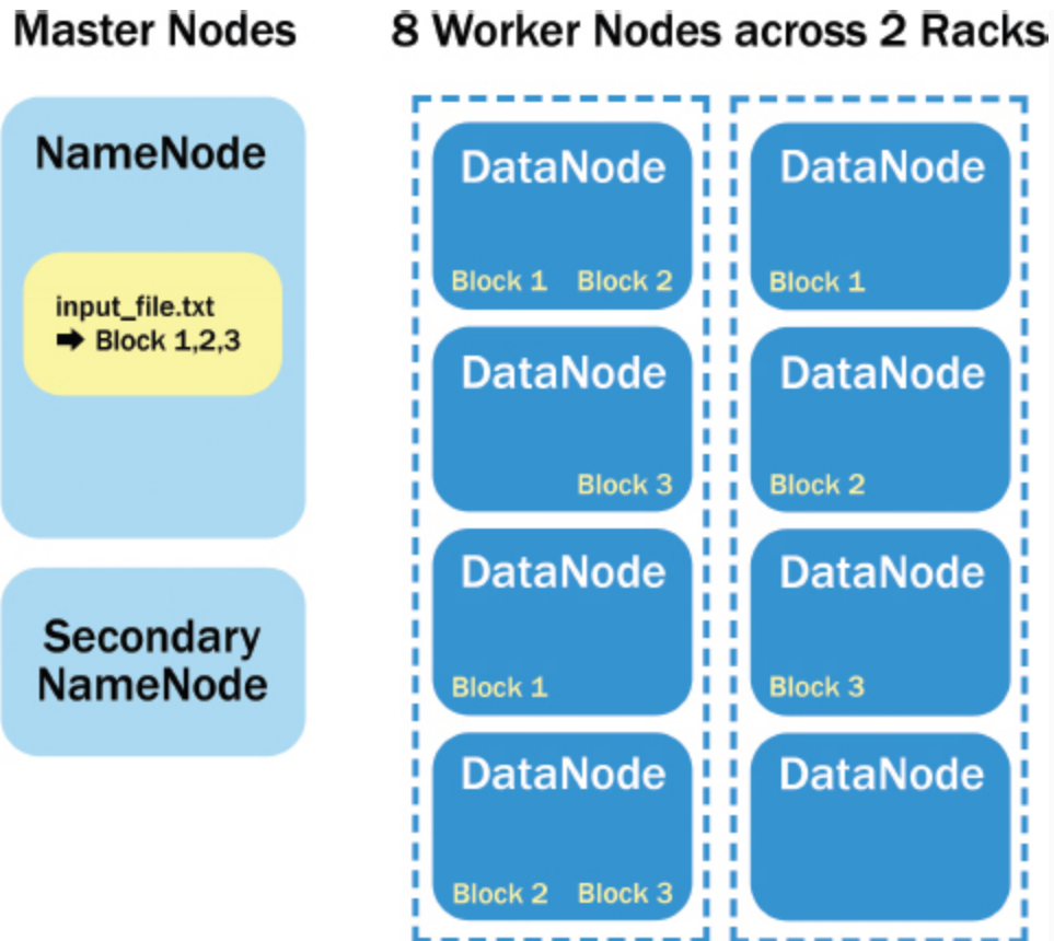
FIGURE 10-2 A file stored in HDFS
