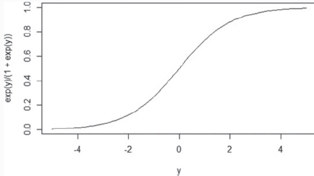
FIGURE 6-14 The logistic function
