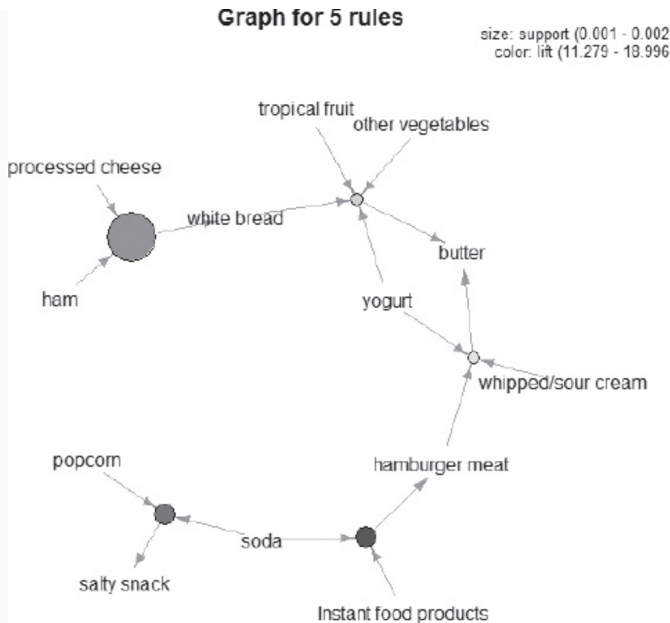
FIGURE 5-6 Graph visualization of the top five rules sorted by lift
