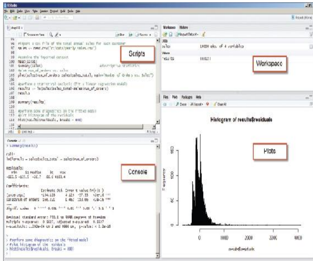
FIGURE 3-3 RStudio GUI
