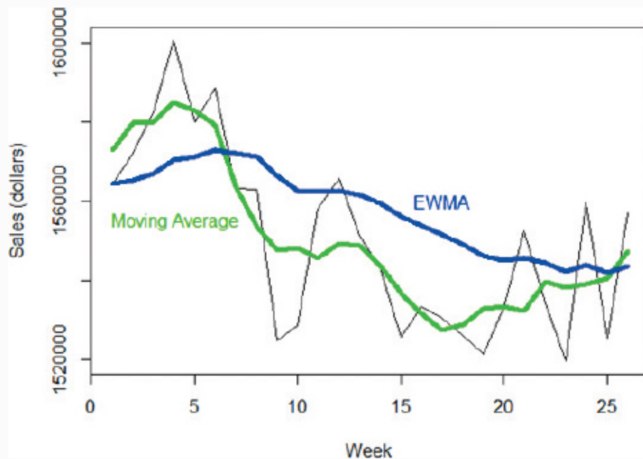
FIGURE 11-4 Weekly sales with moving average and EWMA
