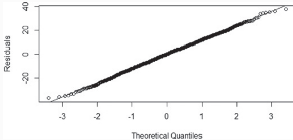
FIGURE 6-12 Q-Q plot of normally distributed residuals
