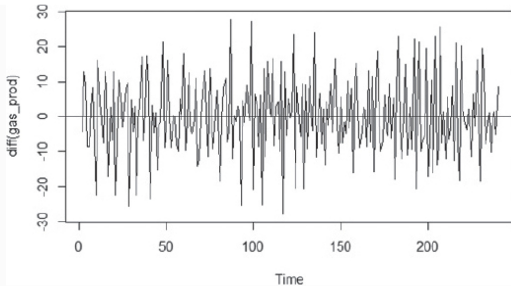
FIGURE 8-12 Differenced gasoline production time series
