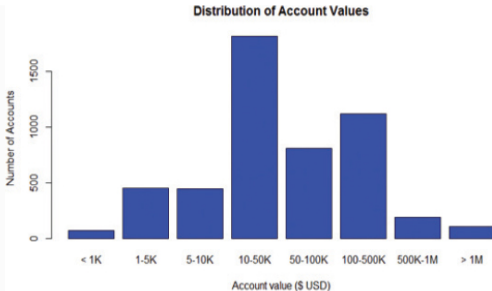
FIGURE 3-21 Histograms are better to show to stakeholders
