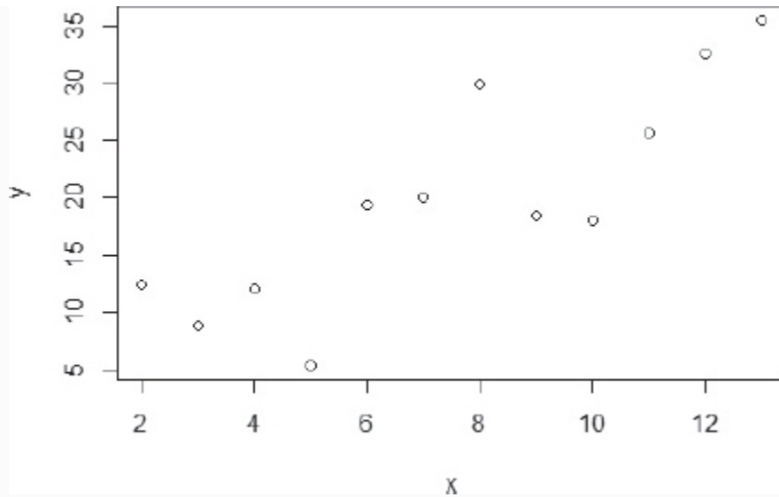
FIGURE 6-1 Scatterplot of y versus x
