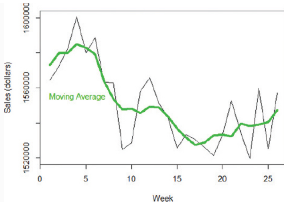
FIGURE 11-3 Weekly sales with moving averages
