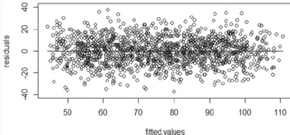
FIGURE 6-6 Residual plot indicating constant variance
