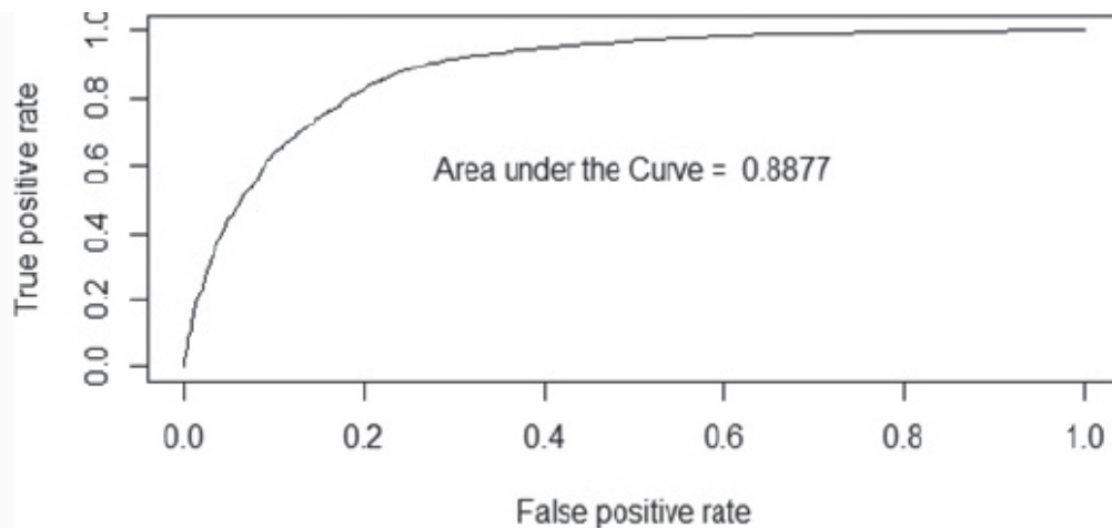
FIGURE 6-15 ROC curve for the churn example
