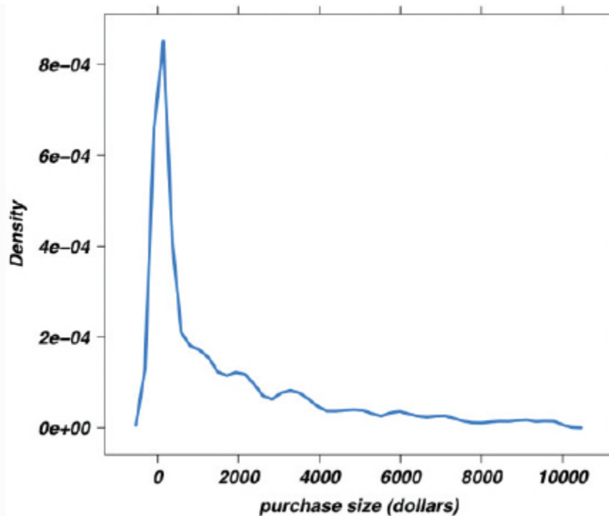
FIGURE 3-27 Density plot of purchase size
