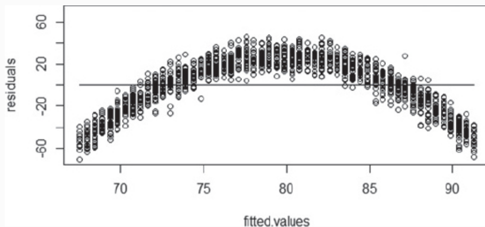
FIGURE 6-7 Residuals with a nonlinear trend
