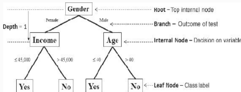
FIGURE 7-1 Example of a decision tree
