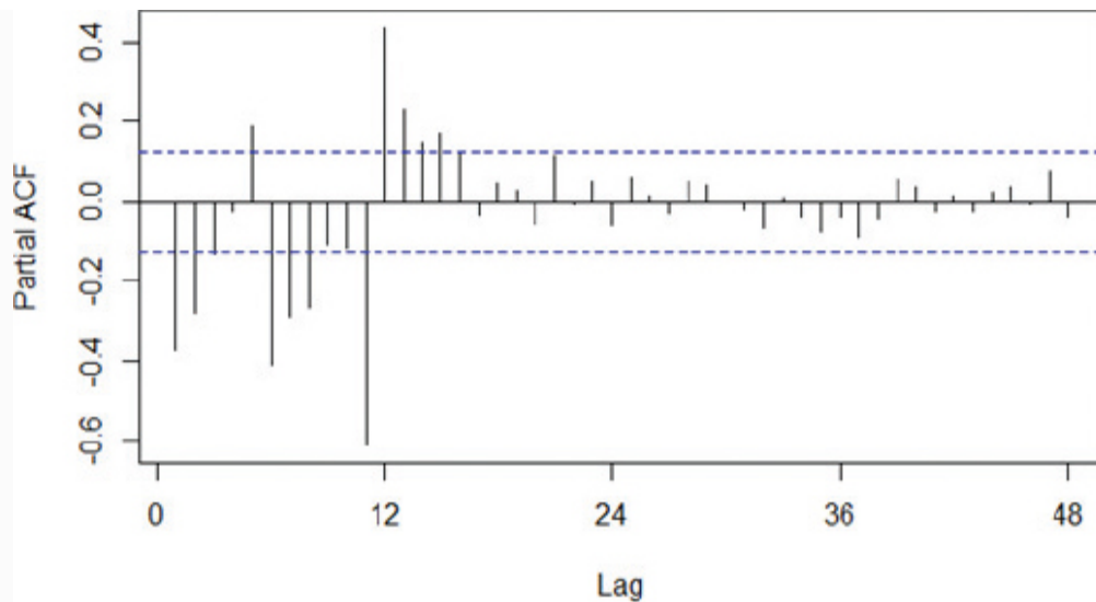
FIGURE 8-14 PACF of the differenced gasoline time series
