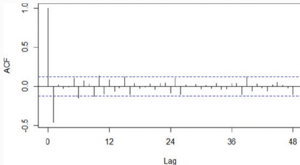
FIGURE 8-15 ACF of residuals from seasonal AR(1) model
