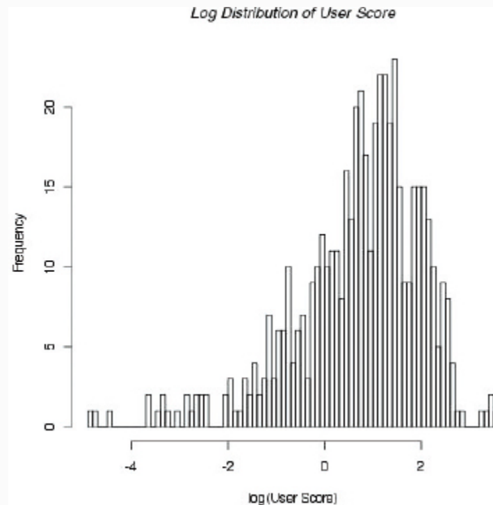
FIGURE 12-20 Frequency distribution with log of user score
