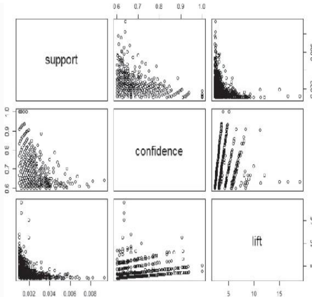
FIGURE 5-4 Scatterplot matrix on the support, confidence, and lift of the 2,918 rules
