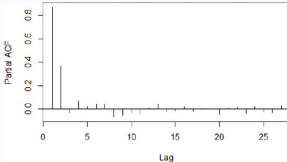
FIGURE 8-4 Partial autocorrelation function (PACF) plot
