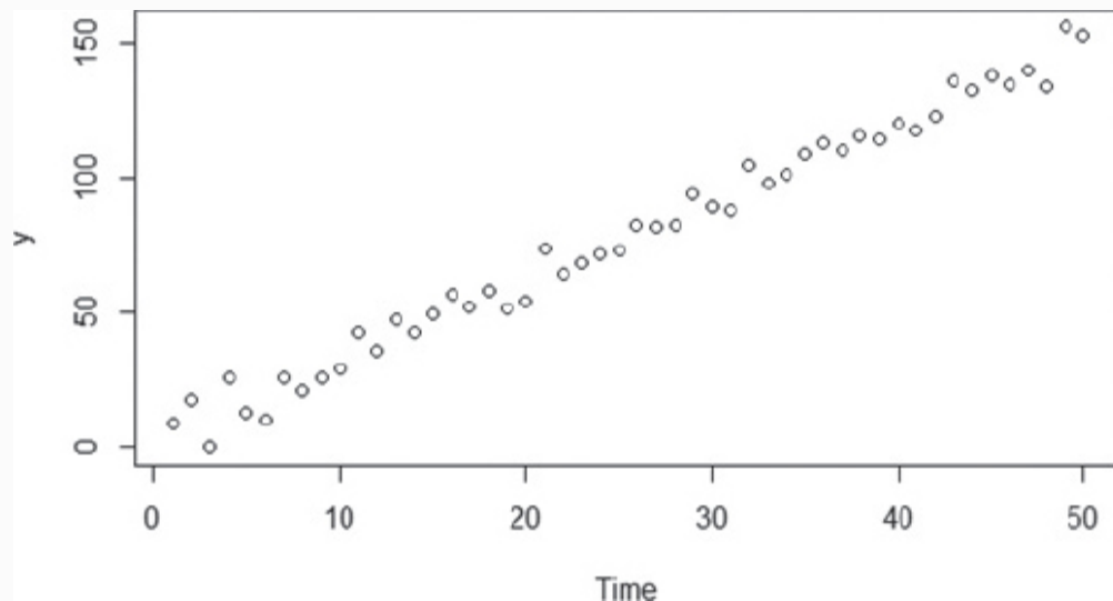
FIGURE 8-7 A time series with a trend
