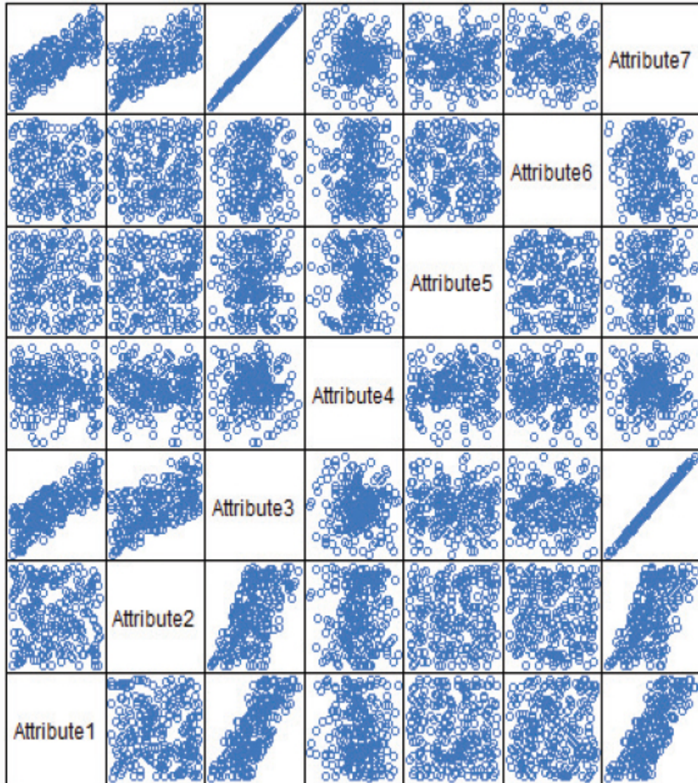
FIGURE 4-10 Scatterplot matrix for seven attributes
