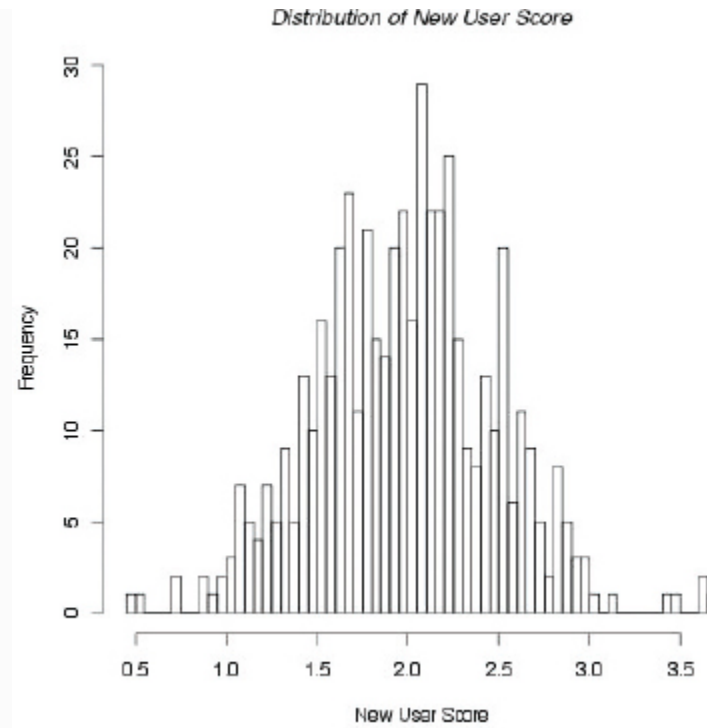
FIGURE 12-21 Frequency distribution of new user scores
