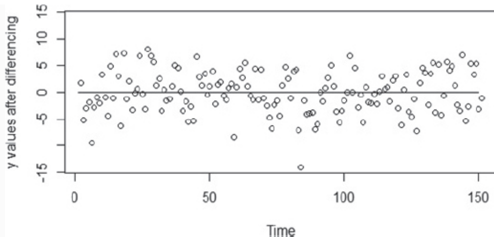
FIGURE 8-9 Detrended time series using differencing
