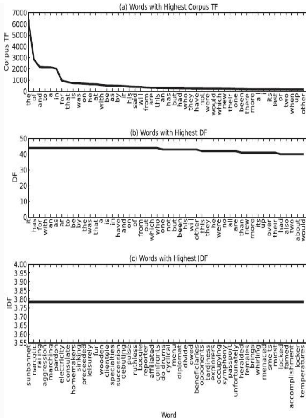
FIGURE 9-3 Words from Brown corpus's news category with the highest corpus TF, DF, or IDF
